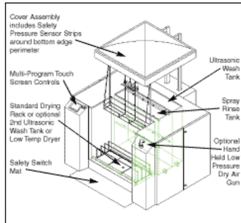
Fig. 1 Model 6000 - Schematic
